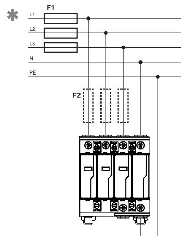
TN-S, TT (3+1)
