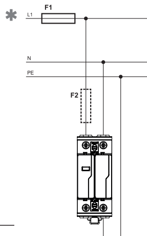
TN-S, TT (1+1)
